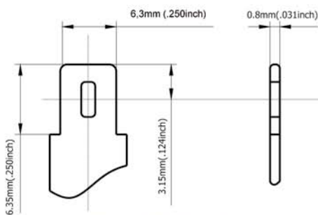
Terminal Dimensions
